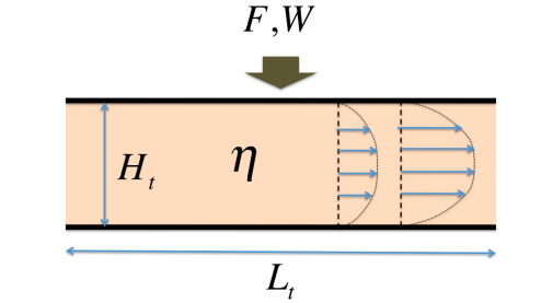
Figure 6. Squeezing a rectangular fluid volume representing an asperity.
