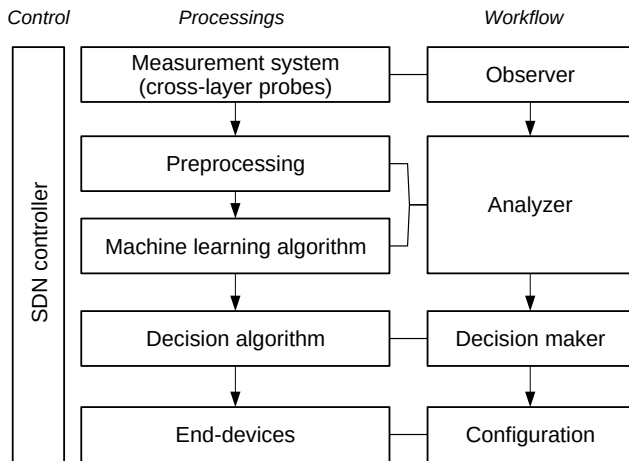
Figure 1. Proposed architecture inspired from CogNet [28].
