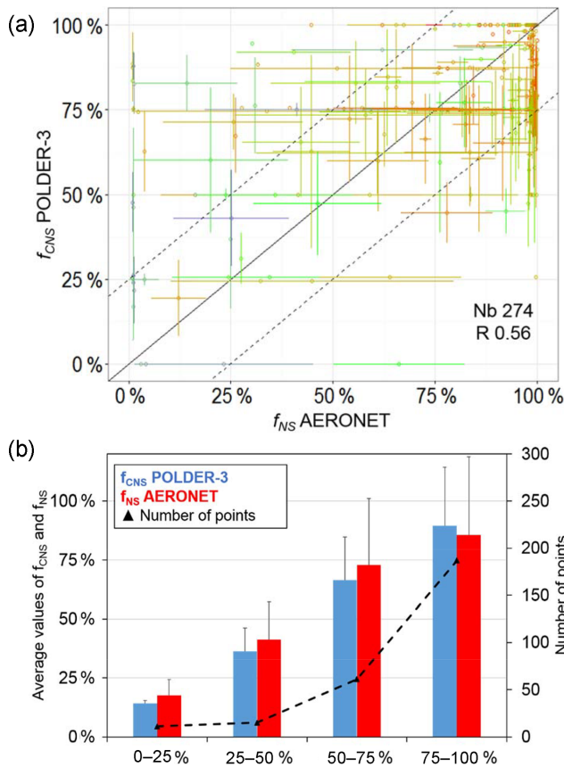
Figure 9. (a) Scatter plot of the fraction of coarse mode optical depth due to non-spherical particles ( f_{\text{CNS}} ) retrieved by POLDER-3 and that of total optical depth ( f_{\text{NS}} ) estimated by AERONET. Values are expressed in percent. As the AERONET f_{\text{NS}} depends on the total aerosol optical depth, only data points for which the measured AOD exceeded 0.10 and the \text{AOD}_{\text{C}} represented more than 30 % of the total AOD are represented. The solid line is the bisector. Dashed lines represent the interval of \pm 25\% of agreement between POLDER-3 f_{\text{CNS}} and AERONET f_{\text{NS}} . (b) Mean and standard deviations of coarse mode optical depth due to non-spherical particles measured by POLDER-3 ( f_{\text{CNS}} , blue) and that of total optical depth estimated by AERONET ( f_{\text{NS}} , red) are classified into four classes: spherical ( f_{\text{CNS}} \leq 25\% ); predominant spherical ( 25\% < f_{\text{CNS}} \leq 50\% ); predominant non-spherical ( 50\% < f_{\text{CNS}} \leq 75\% ); non-spherical ( 75\% < f_{\text{CNS}} \leq 100\% ). Values are expressed in percentages. Only AERONET data points for which the \text{AOD} > 0.10 and \text{AOD}_{\text{C}}/\text{AOD} > 0.30 are represented. The black triangles represent the number of points in each class (the dashed curve is represented for increased readability).
