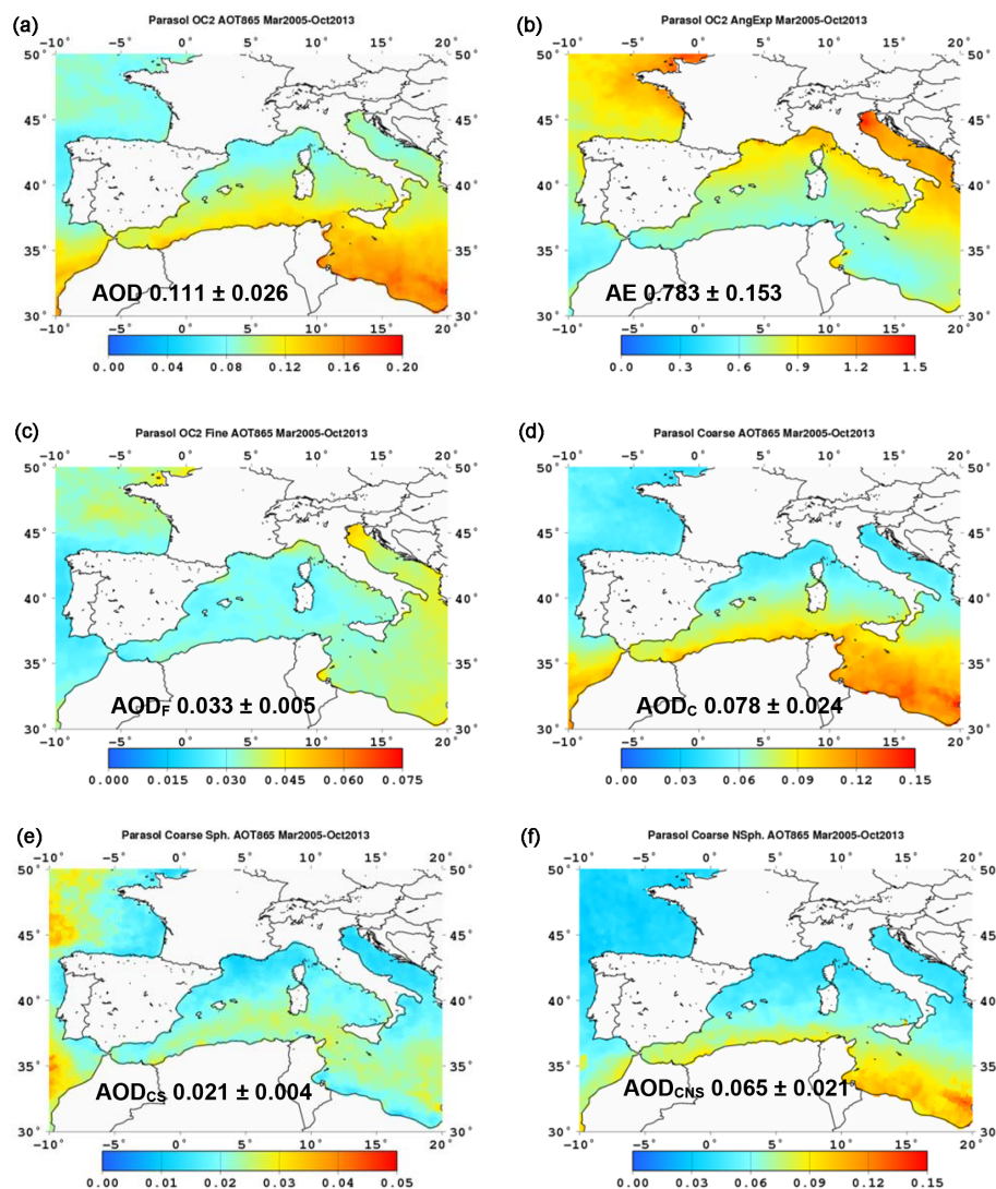
Figure 11. Regional maps for AOD, AE, AOD F , AOD C , AOD CS , and AOD CNS (from left to right and top to bottom) retrieved by POLDER-3 for the period March 2005–October 2013. Mean and standard deviations over the whole marine area of the window are also shown.
