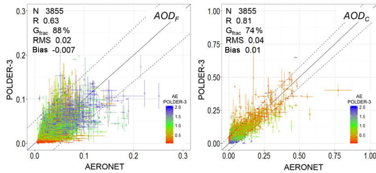
Figure 4. Scatter plots of daily AOD_F and AOD_C retrieved by POLDER-3 at 865 nm as a function of coincident AERONET values at 870 nm for the 17 sites of the western Mediterranean Sea. The solid line is the bisector. The dashed lines represent the limits indicated by the G_{frac} parameter. The characteristics of the linear correlation (number of points N , correlation coefficient R , G_{frac} , RMSE, and bias) are also reported. Note that, as discussed in Sect. 2.1 and 2.2, the definitions of AOD_F and AOD_C by POLDER-3 and AERONET are not the same.
