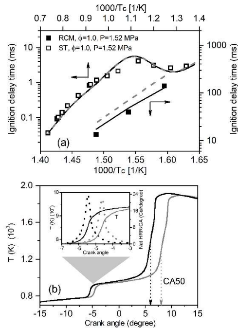
Figure 40: Effect of third O 2 addition reactions on IDTs and combustion phasing of n -hexane: (a) Shock tube (top-left axes), rapid compression machine (bottom-right axes) IDTs of n -hexane/air mixtures. Symbols are experimental data by Zhang et al. [282]. Black solid lines and grey dashed lines are simulation with [326] and without [282] third O 2 addition reactions. (b) Temperature dependence with crank angle during n -hexane/air mixtures in an HCCI engine ignition. Black and grey lines are simulation by model with and without third O 2 addition reactions, respectively. Net heat release rate (HRR) per crank angle and zoomed temperature profiles shown in inset – reproduced from Ref. [326] with permission from Elsevier.
