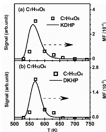
Figure 39: Temperature-dependent profiles of C 7 H 14 O 5 and C 7 H 12 O 4 intermediates in 2-methylhexane low-temperature oxidation. Symbols are experimental measurements; lines are simulated mole fractions of KDHP (C 7 H 14 O 5 ) and DKHP (C 7 H 12 O 4 ). Mole fractions refer to all isomers. Experimental signal and model prediction are scaled to match - adapted from Ref. [252].
