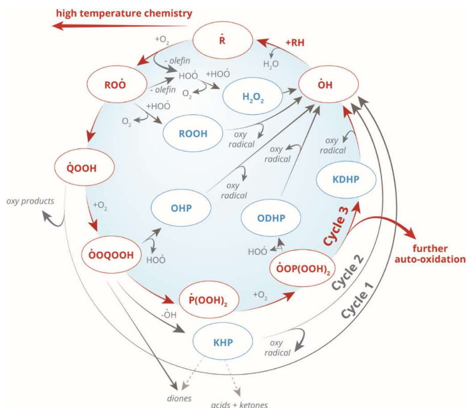
Figure 46: Updated reaction scheme for alkane low-temperature oxidation.
