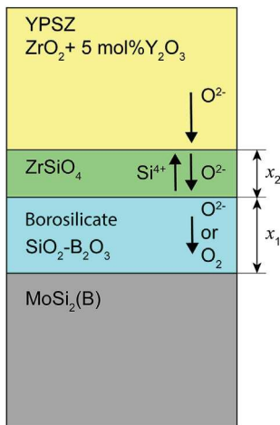
Fig. 10. Schematic of the transport phenomena associated with the formation of borosilicate and ZrSiO 4 layers in the YPSZ - MoSi 2 (B) interdiffusion couples when exposed to high temperatures in air.
