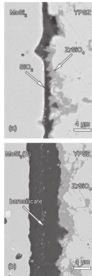
Fig. 5. SEM backscattered electron images of cross-section of (a) YPSZ – MoSi_2 and (b) YPSZ – MoSi_2(B) interdiffusion couples after annealing for 96 h at 1100 °C in laboratory air. A silica layer (a) or borosilicate layer (b) is developed due to oxidation of MoSi_2 and MoSi_2(B) , respectively. The very small bright phase at the edge of MoSi_2 and MoSi_2(B) belongs to Mo_5Si_3 . In between the silica or borosilicate layer and the YPSZ, zircon ( ZrSiO_4 ) is formed.
