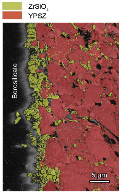
Fig. 7. Phase map of YPSZ-MoSi 2 (B) interdiffusion couple after annealing at 1200 °C in laboratory air for 96 h, showing the ZrSi 4 formation at the YPSZ – SiO 2 + 5 at.% B interface and along grain boundaries of YPSZ as obtained by SEM – EBSD of a cross section.
