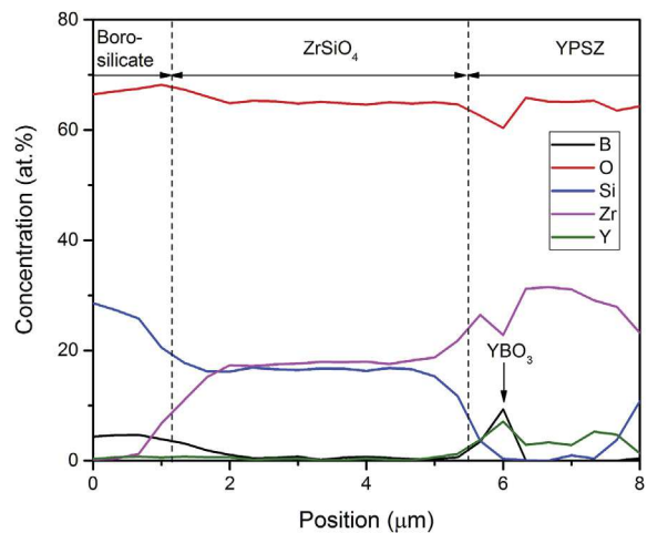
Fig. 6. Chemical composition profile across the YPSZ – MoSi_2(B) interdiffusion couple after annealing at 1200 °C in laboratory air for 96 h, as obtained with EPMA. Error less than 0.5 at.% for each element.
