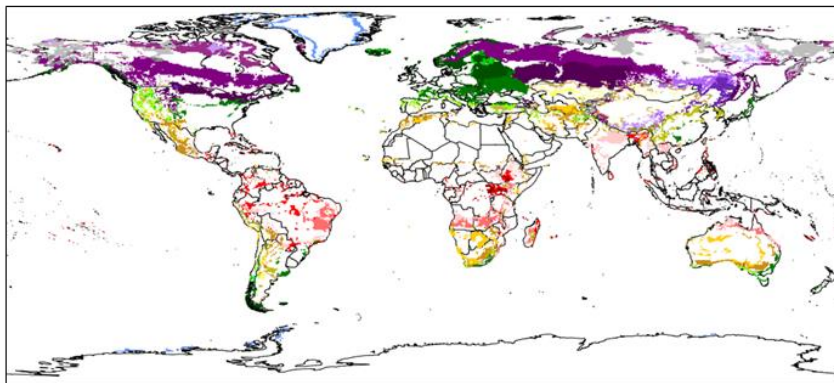
Figure 5: Köppen classification results at a global scale. (a) historical run for 1986-2005 and (b) RCP8.5 run for 2041-2060, obtained using the IPSL-CM5A-LR bias-corrected model.
