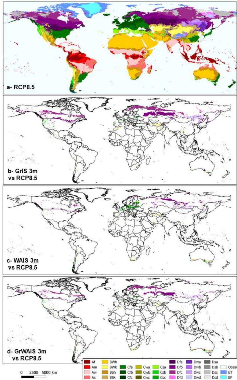
Figure 9: Köppen classification results showing temperature-related sub-group changes (3rd letter on the Köppen nomenclature) between (a) the RCP8.5 and (b) the GrIS 3m, (c) the WAIS 3m and (d) the GrWAIS 3m scenarios for the period 2041-2060. Colors represent sub-group shifts, areas in white being unaffected by sub-group changes. Other scenarios (0.5, 1 and 1.5 m water input) are in the supplementary materials.
