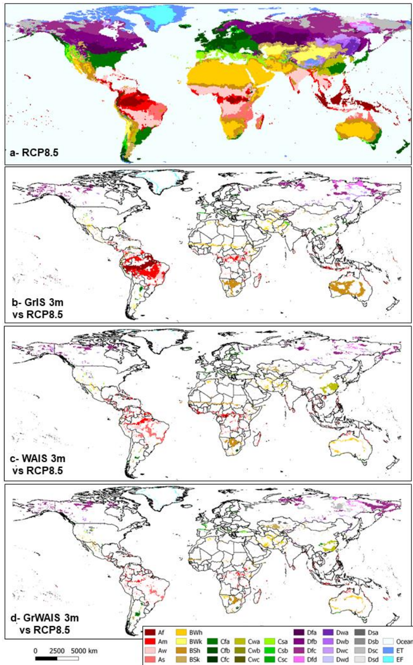
Figure 8: Köppen classification results showing precipitation-related sub-group changes (3rd letter on the Köppen nomenclature) between (a) the RCP8.5 and (b) the GrIS 3m, (c) the WAIS 3m and (d) the GrWAIS 3m scenarios for the period 2041-2060. Colors represent sub-group shifts, areas in white being unaffected by sub-group changes. Other scenarios (0.5, 1 and 1.5 m water input) are in the supplementary materials.
