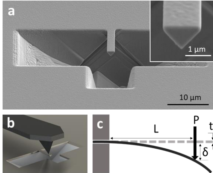
Figure 1 - (a) SEM image of a MoS 2 micro-cantilever beam FIB milled in the 1.1 μm thick MoS 2 coating, the inset is a zoomed in image on the beam cross section. (b) 3D schematic representation of the bending test using AFM, at scale. (c) schematic of the deflection test performed on the beam using AFM.
