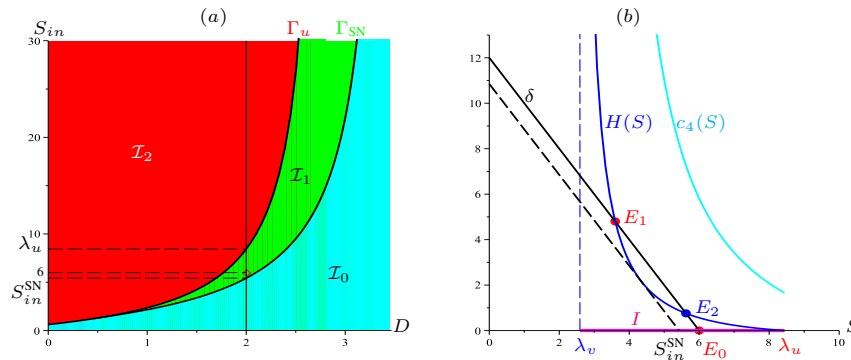
Figure 3 – (a) The operating diagram of (1) when case (7) holds. (b) The existence and stability of steady states corresponding to the diamond point (D, S_{in}) = (2, 6) \in \mathcal{I}_1 .
