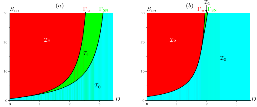
Figure 2 – Effect of mortality on the operating diagram: (a) m_u = 0.7 (b) m_u = 50 .
