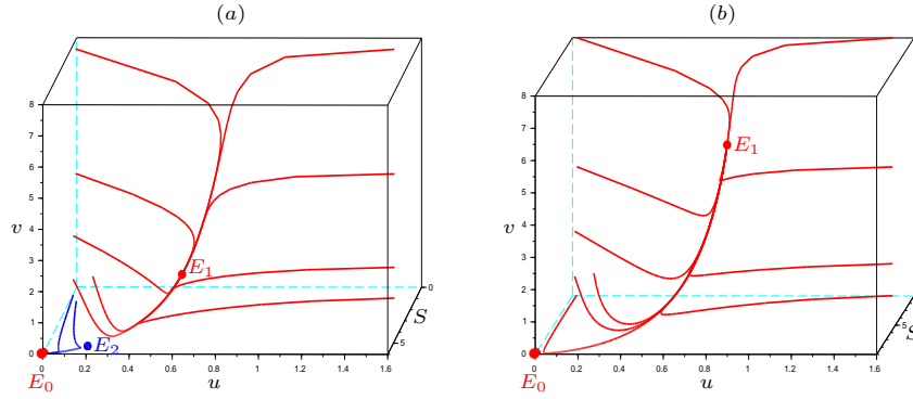
Figure 5. The trajectories of system (1) in three-dimensional space (S, u, v) (a) the bi-stability of E_0 and E_1 when (D^*, S_{in}^*) = (2, 6) \in \mathcal{I}_1 . (b) Global convergence to E_1 when (D^*, S_{in}^*) = (2, 9) \in \mathcal{I}_2 .
