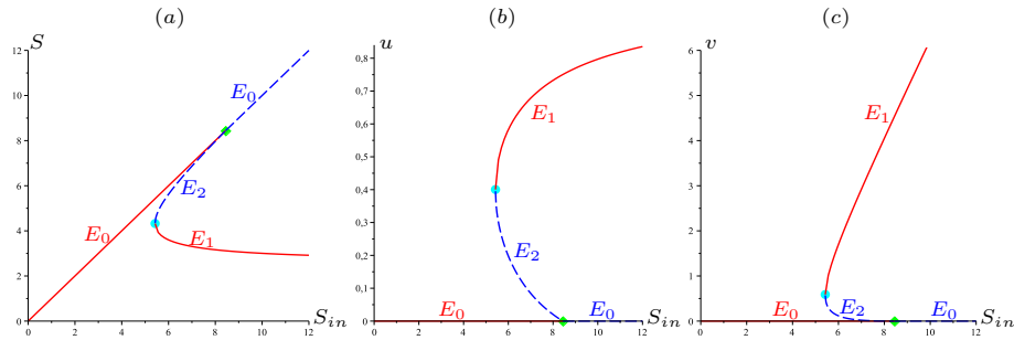
Figure 6. One-parameter bifurcation diagrams for fixed D = 2 showing the effect on the components S , u and v of all steady states as S_{in} varies. Blue dashed curves corresponds to unstable steady states and red solid curves to the stable steady states. The green solid diamonds represent the transcritical bifurcations of E_0 and E_2 while the cyan solid circles represent the saddle-node bifurcations of E_1 and E_2 .
