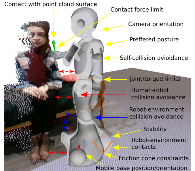
Fig. 1: Safe and feasible humanoid robot posture for pMRI.
