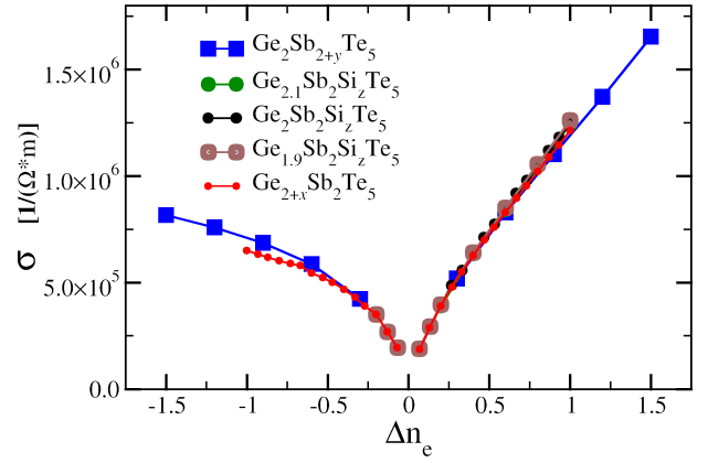
FIG. 11. Conductivity of \text{Ge}_{2+x}\text{Sb}_{2+y}\text{Si}_z\text{Te}_5 crystals as a function of \Delta n_e , the difference in their number of p-valence electrons per formula unit with respect to \text{Ge}_2\text{Sb}_2\text{Te}_5 .
