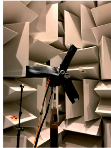
Figure 13. Experimental set-up in the anechoic chamber used to validate the ISO standard. The five components aerodynamic balance is below the motor driving the rotor.
