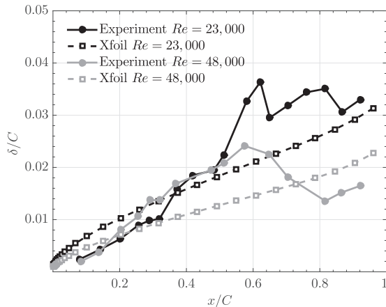
Figure 2. Boundary layer thickness on a NACA 0012 at Reynolds numbers Re = 23,000 and Re = 48,000 and a 6^\circ angle of attack between Xfoil prediction and experiments by Kim et al. 22
