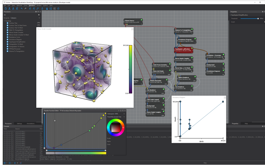
Fig. 12 Integration of TTK in a software ecosystem other than VTK/ParaView: Inviwo [23], a software framework for the rapid prototyping of visualizations, written in C++ and exploiting modern graphics hardware. This example shows the topological analysis with the Morse-Smale complex (with persistence-driven data pre-simplification) of charge densities in iron oxide [22].
