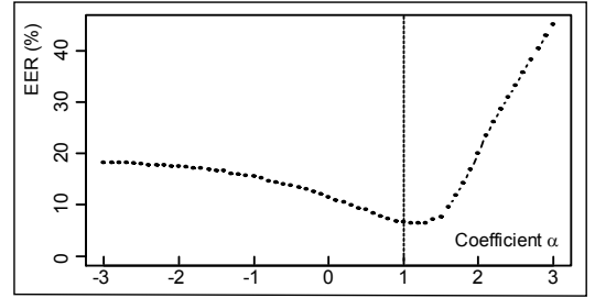
Fig. 2. Fusion v_1 \cdot v_2 - \alpha (v_1 \cdot A v_2) of initial and binary eigenvectors matrix scores: coefficient \alpha and resulting EER%
