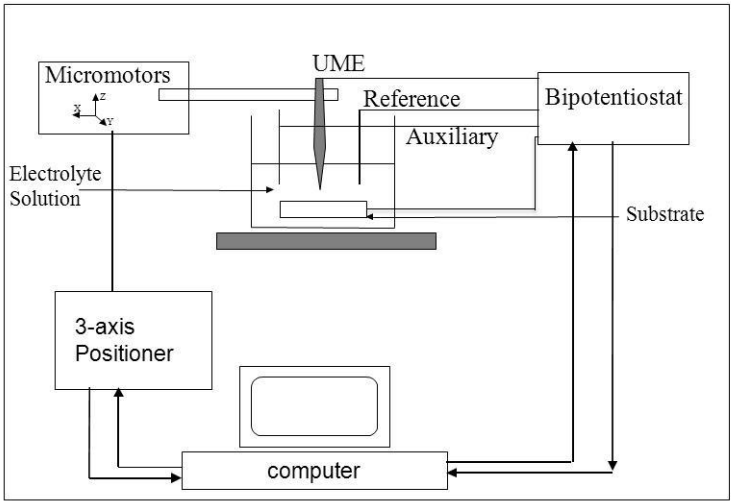
Figure 1 An illustration of an SECM instrument.
