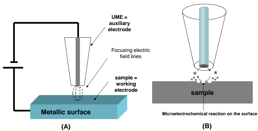
Figure 7. Schematic representation of the direct mode (A) and the feedback mode (B) of the SECM for the localized modification of the substrate surface.
