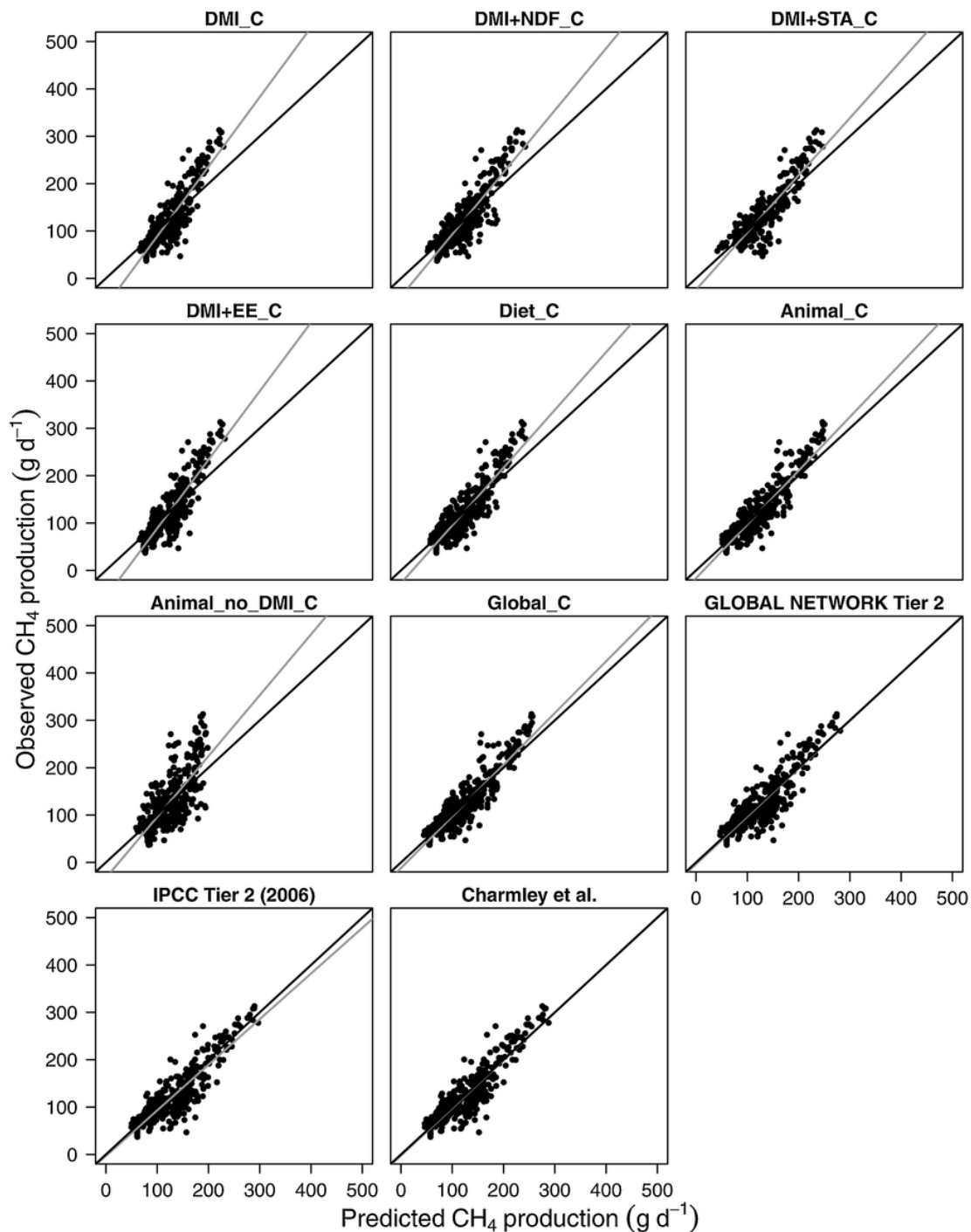
Fig. 5. Observed vs. predicted plots for North American higher-forage methane emission ( \text{g d}^{-1} \text{ animal}^{-1} ) prediction equations for the different categories, viz., dry matter intake (DMI_C), dry matter intake and neutral detergent fiber (DMI + NDF_C), dry matter intake and starch (DMI + STA_C), dry matter intake and ether extract (DMI + EE_C), dietary (Diet_C), animal (Animal_C), animal without DMI (Animal_no_DMI_C), global (Global_C), GLOBAL NETWORK Tier 2 (2006), IPCC Tier 2 (2006), and the extant Charmley et al. (2016) equation. The gray and black solid lines represent the fitted regression line for the relationship between observed and predicted values, and the identity line ( y = x ), respectively.
