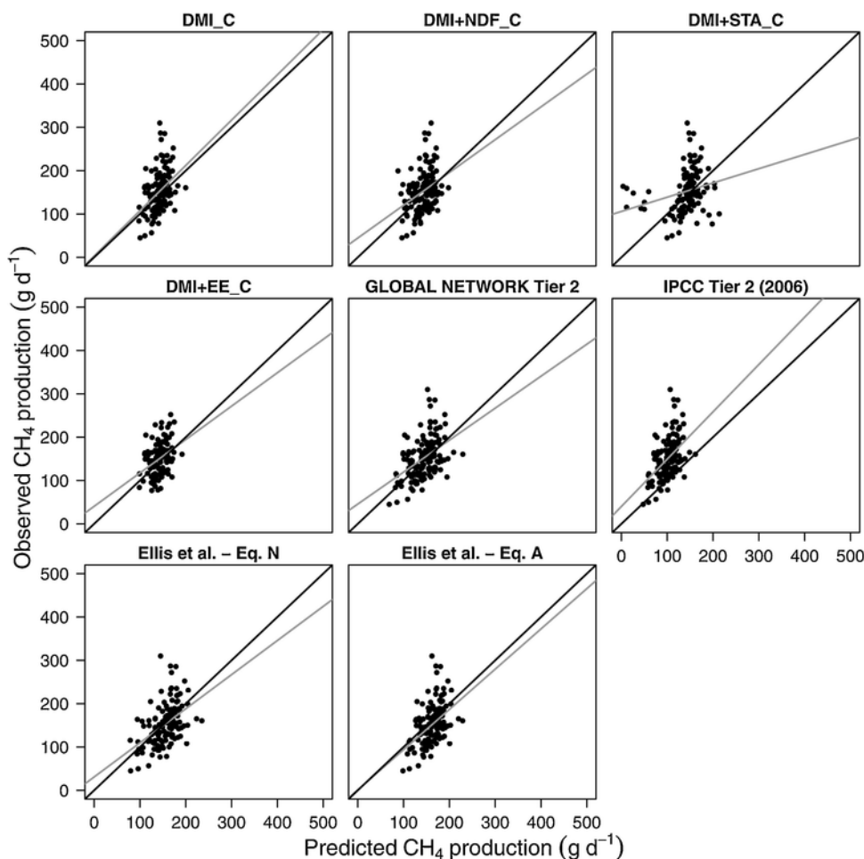
Fig. 3. Observed vs. predicted plots for lower-forage methane emission ( \text{g d}^{-1} \text{ animal}^{-1} ) prediction equations for the different categories, viz., dry matter intake (DMI_C), dry matter intake and neutral detergent fiber (DMI + NDF_C), dry matter intake and starch (DMI + STA_C), dry matter intake and ether extract (DMI + EE_C), GLOBAL NETWORK Tier 2, IPCC Tier 2 (2006), and the extant Ellis et al. (2009) equations. The gray and black solid lines represent the fitted regression line for the relationship between observed and predicted values, and the identity line ( y = x ), respectively.
