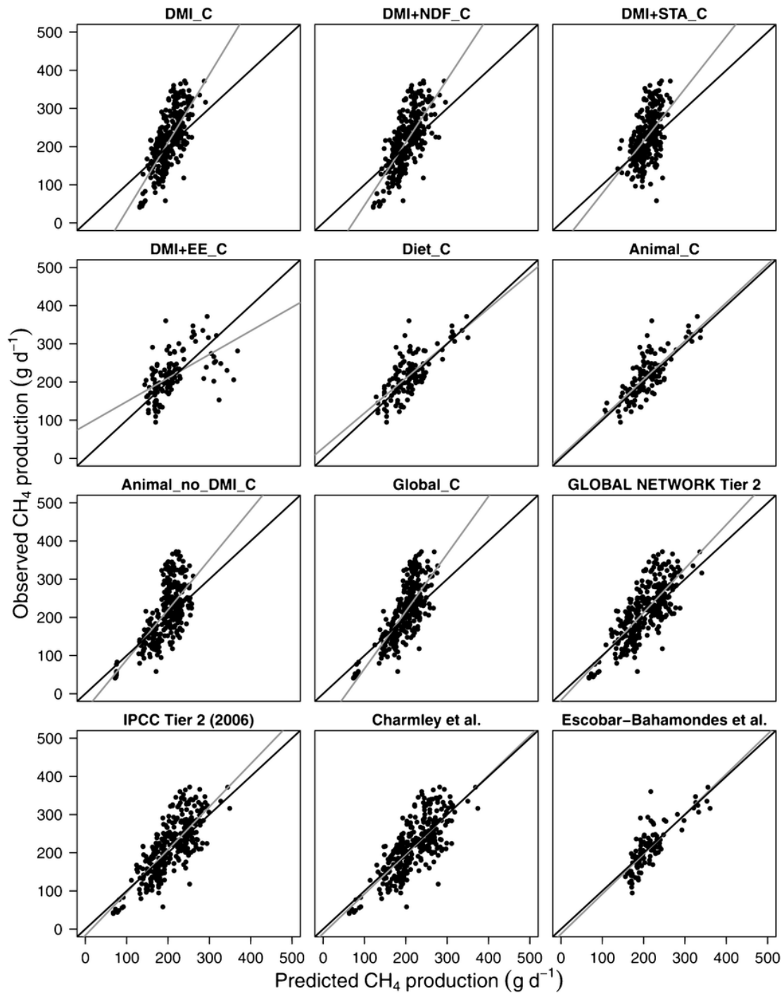
Fig. 4. Observed vs. predicted plots for European higher-forage methane emission ( \text{g d}^{-1} \text{ animal}^{-1} ) prediction equations for the different categories, viz., dry matter intake (DMI_C), dry matter intake and neutral detergent fiber (DMI + NDF_C), dry matter intake and starch (DMI + STA_C), dry matter intake and ether extract (DMI + EE_C), dietary (Diet_C), animal (Animal_C), animal without DMI (Animal_no_DMI_C), global (Global_C), GLOBAL NETWORK Tier 2, and IPCC Tier 2 (2006), and the extant Charmley et al. (2016) and Escobar-Bahamondes et al. (2017) equations. The gray and black solid lines represent the fitted regression line for the relationship between observed and predicted values, and the identity line ( y = x ), respectively.
