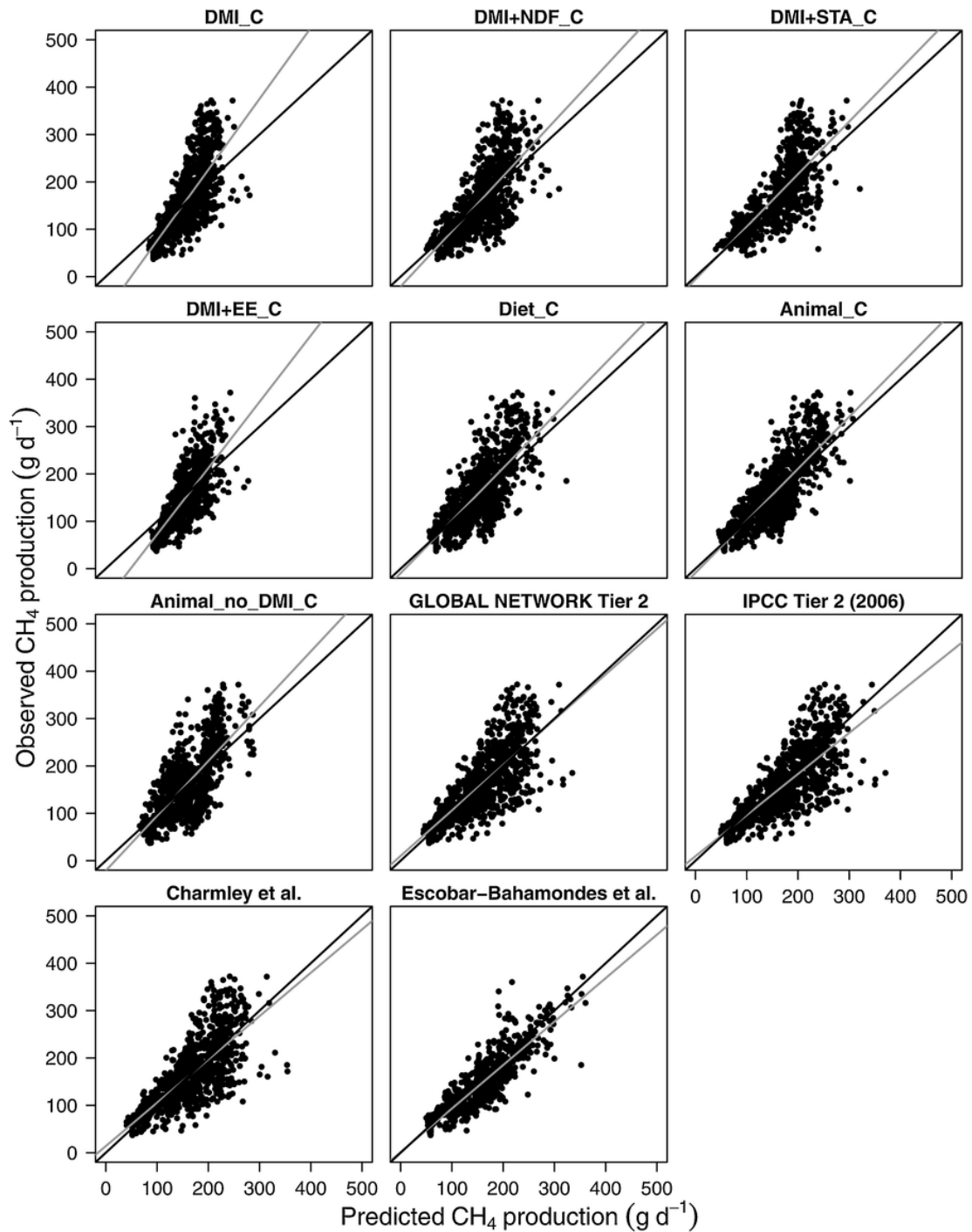
Fig. 1. Observed vs. predicted plots for all-data methane emission ( \text{g d}^{-1} \text{ animal}^{-1} ) prediction equations for the different categories, viz., dry matter intake (DMI_C), dry matter intake and neutral detergent fiber (DMI + NDF_C), dry matter intake and starch (DMI + STA_C), dry matter intake and ether extract (DMI + EE_C), diet (Diet_C), animal (Animal_C), animal without DMI (Animal_no_DMI_C), GLOBAL NETWORK Tier 2, IPCC Tier 2 (2006), and the extant Charmley et al. (2016) and Escobar-Bahamondes et al. (2017) equations. The gray and black solid lines represent the fitted regression line for the relationship between observed and predicted values, and the identity line ( y = x ), respectively.
