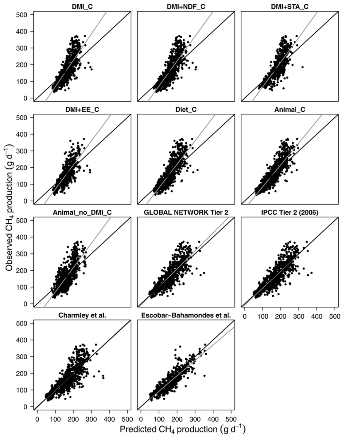
Fig. 2. Observed vs. predicted plots for higher-forage methane emission ( \text{g d}^{-1} \text{ animal}^{-1} ) prediction equations for the different categories, viz., dry matter intake (DMI_C), dry matter intake and neutral detergent fiber (DMI + NDF_C), dry matter intake and starch (DMI + STA_C), dry matter intake and ether extract (DMI + EE_C), diet (Diet_C), animal (Animal_C), animal without DMI (Animal_no_DMI_C), GLOBAL NETWORK Tier 2, IPCC Tier 2 (2006), and the extant Charmley et al. (2016) and Escobar-Bahamondes et al. (2017) equations. The gray and black solid lines represent the fitted regression line for the relationship between observed and predicted values, and the identity line ( y = x ), respectively.
