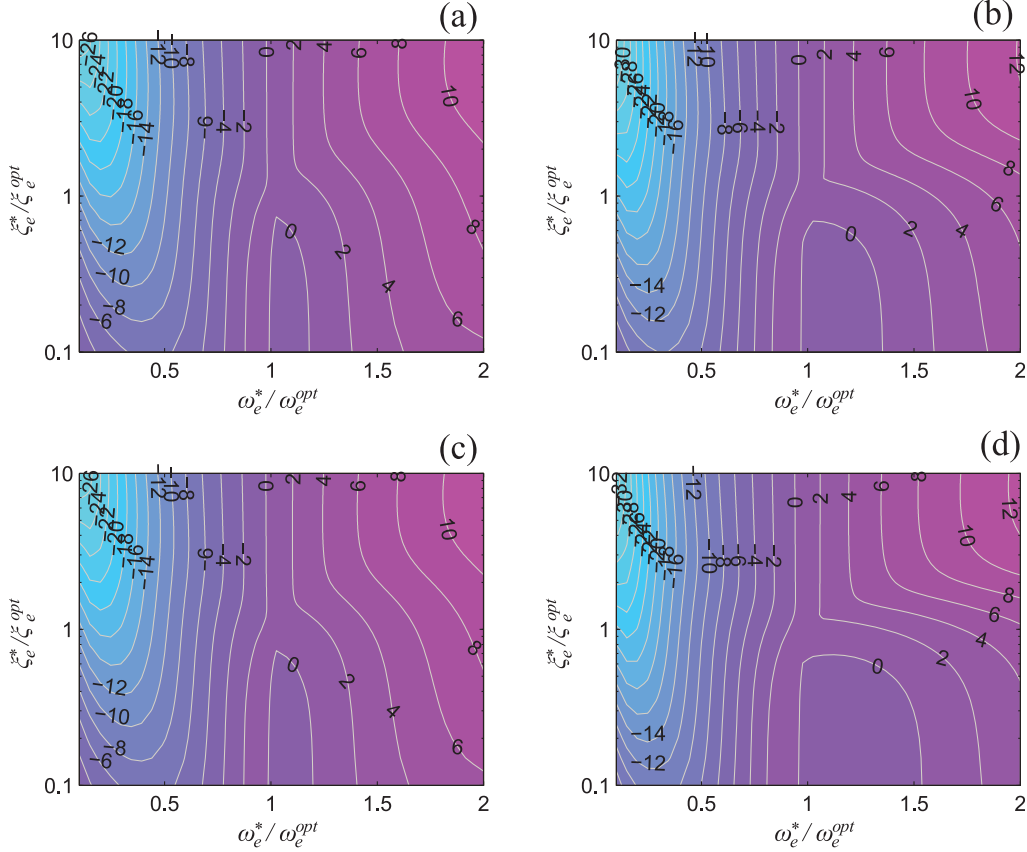
Figure 13. A_{\text{dB,num}}^{*,\text{S,P}} - A_{\text{dB,num}}^{*,\text{P,P}} for a system with \xi_i = 0.1\% and k_i = 0.2 : (a) \tilde{k}_i = 0.4 and (b) \tilde{k}_i = 0.6 . A_{\text{dB,num}}^{*,\text{S,S}} - A_{\text{dB,num}}^{*,\text{P,S}} for a system with \xi_i = 0.1\% and k_i = 0.2 : (c) \tilde{k}_i = 0.4 and (d) \tilde{k}_i = 0.6 .
