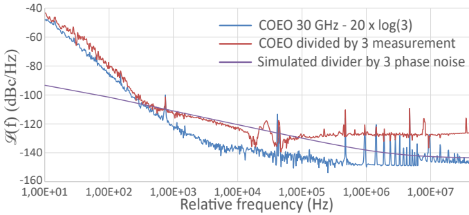
Fig. 6. COEO divided by 3 phase noise : Noise floor vs measured vs simulated
