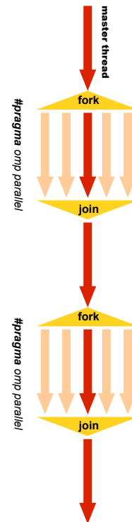
Figure 4: OpenMP is based on a fork-join model
