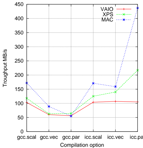
Figure 11: fdelay8.dsp benchmark
