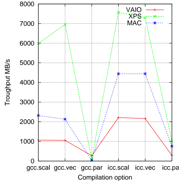
Figure 6: Copy1.dsp benchmark
