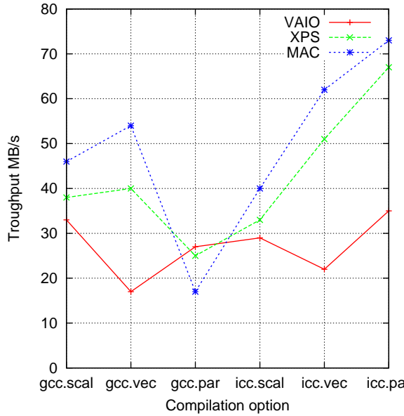
Figure 9: Karplus32.dsp benchmark
