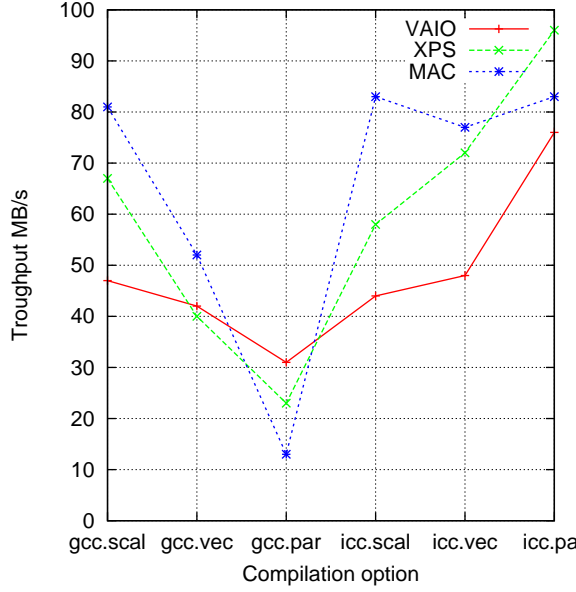
Figure 8: Freeverb.dsp benchmark
