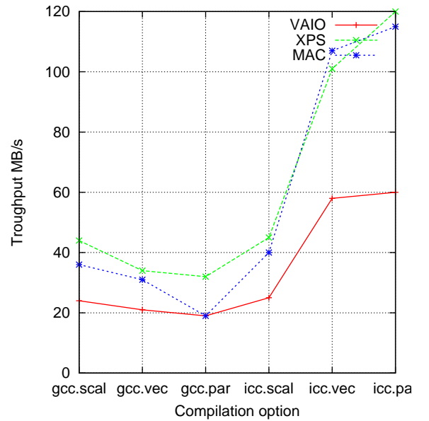
Figure 10: mixer.dsp benchmark
