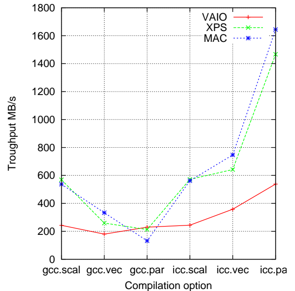
Figure 13: rms8.dsp benchmark
