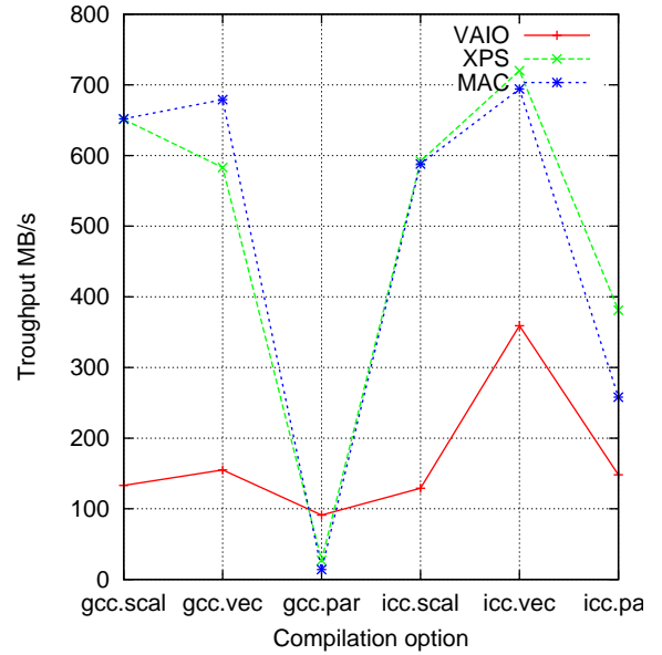
Figure 12: rms.dsp benchmark
