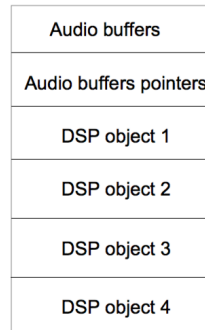
Figure 7: Wasm memory block layout for a polyphonic DSP (here with 4 voices)
