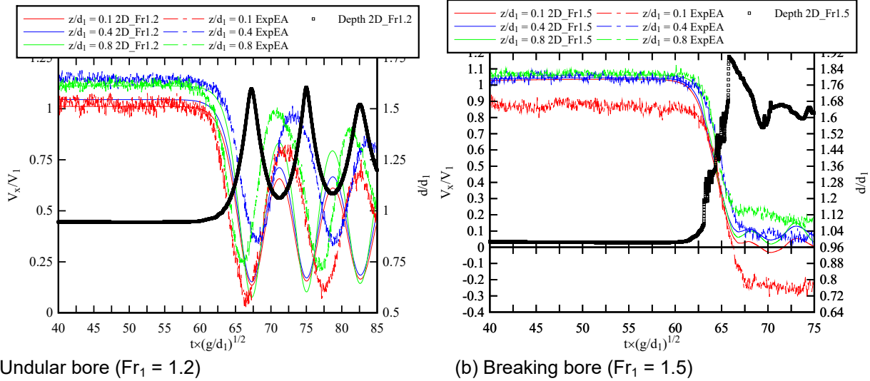
(a) Undular bore ( Fr_1 = 1.2 ) (b) Breaking bore ( Fr_1 = 1.5 ) Figure 4. Dimensionless time-variations of longitudinal velocity for undular and breaking bores of Fr_1 = 1.2 and 1.5 , respectively; Comparisons between numerical simulation (2D_Fr) and ensemble-averaged experimental data (ExpEA).
