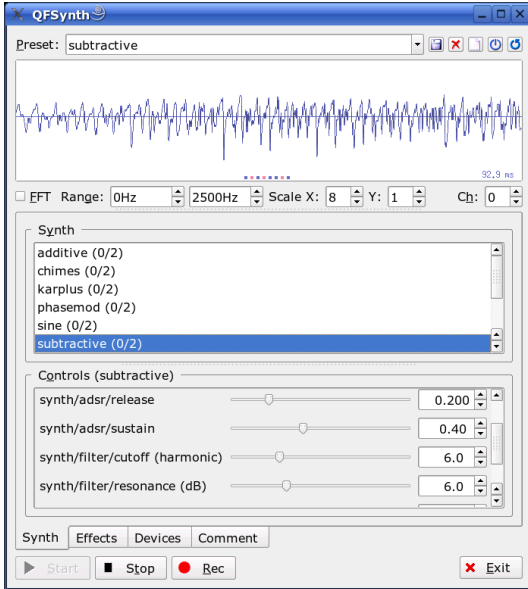
Figure 6: QFSynth program
