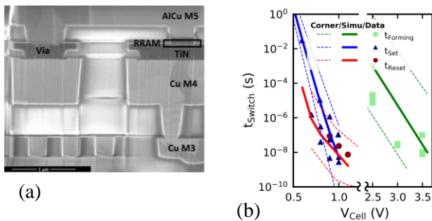
Fig. 1. (a) TEM cross section of TiN/HfO 2 /Ti/TiN OxRAM [21]. (b) Measured switching times t_{\text{Forming}} , t_{\text{Set}} and t_{\text{Reset}} versus applied programming voltage V_{\text{Cell}} (symbols), and the corresponding simulation results with corners (lines). Experimental data were measured on the adopted OxRAM technology in [9,22].
