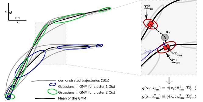
Fig. 8: Left: demonstrated trajectories (light gray) and the two GMMs. Right: Relevant variables for computing g(\mathbf{x}_r; s_{vm}) .
