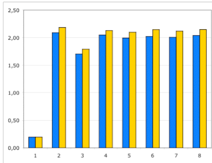
Figure 7: Compared paired pop/push operation cost in microseconds for 1 to 8 concurrent tasks on intel1.
