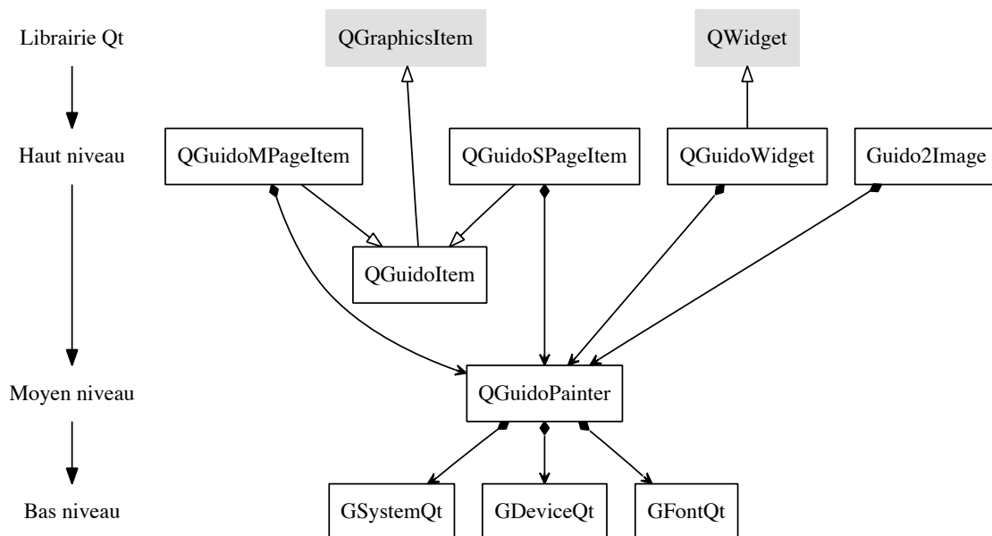
Figure 4. Diagramme des classes GuidoQt
