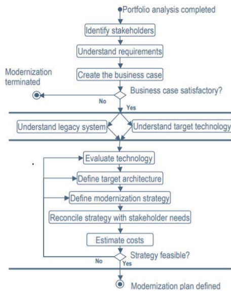
Fig. 4. A systematic framework for legacy program module modernization, adopted from [6]
