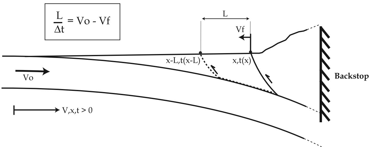
Figure 12. Sketch illustrating how the rate of sediment accretion relates to the velocities defined in Figure 1. Accretion of foreland sediments into the foothills accommodates the relative motion between the footwall and the mountain belt, and more precisely between the foreland and the front of the range. While a slice of sediments with a length L is accreted at time t(x - L) , the frontal fault, which also initiated by accretion at time t(x) , migrates L away from the orogen. However, internal shortening of the new thrust sheet will eventually bring the front back to its initial position relative to the backstop. Therefore, by retrieving the present distance between faults within the WF and by accounting for the finite shortening of the thrust sheets, this accretion rate, which also corresponds to the relative velocity V_o - V_f , can be easily assessed.
