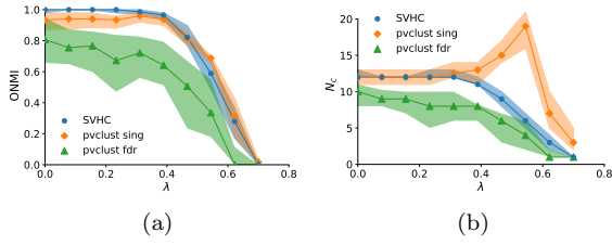
FIG. 4. (a) Overlapping normalized mutual information (ONMI) between the true hierarchical partition of the benchmark of Fig. 2 with N = 100 and M = 500 and the hierarchical partition obtained with SVHC, Pvcust "single" or Pvcust "FDR" as a function of the noise parameter \lambda . (b) Number of statistically validated clusters detected by the algorithms as a function of the noise parameter \lambda . Points are the median computed in 100 independent realizations. The color band highlights the interval between the 25 and the 75 percentile. In our numerical experiments, we simulate 1000 bootstrap replicas both for the SVHC and the Pvcust algorithm.
