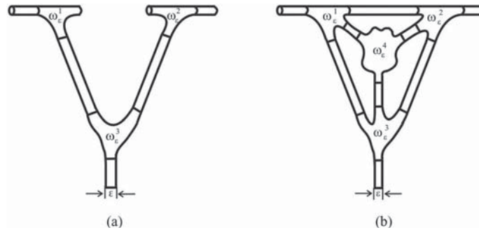
FIG. 1. Fluid flow domains: Tube structures.
