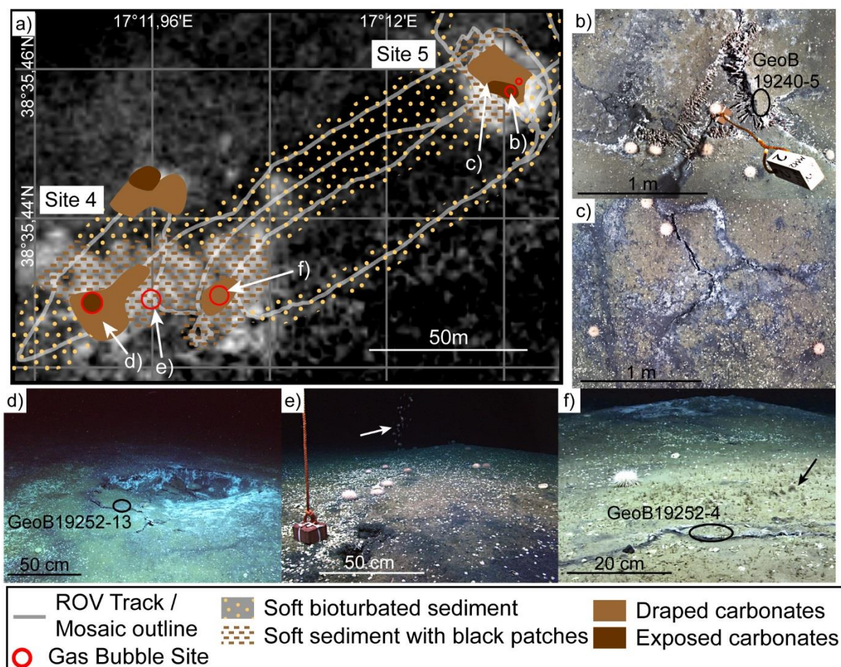
Figure 5. Sites 4 and 5 (location in Fig. 1); a: Map view of AUV-borne backscatter (white is high backscatter) superimposed with seafloor categories mapped along the ROV track and the location of a photomosaic at Site 5; visually identified gas bubble sites; b: Detail of photomosaic at Site 5 showing a ruptured mound releasing gas bubbles (see also supplementary video S4) and tube worms underneath the carbonate slabs; c: Detail of photomosaic at Site 5 showing white microbial mats between carbonate pavements next to the ruptured mound; d: Collapse structure at Site 4; e: Gas bubbles (white arrow) rising from black sediment (note holes from push-core sediment sampling next to red marker) and partially sealed mound in the background; f: Gas bubble release (black arrow) from a fracture in carbonate pavement (black circle marks GeoB-No. of carbonate sample) with partially sealed carbonate mound (note white microbial mats on top).
