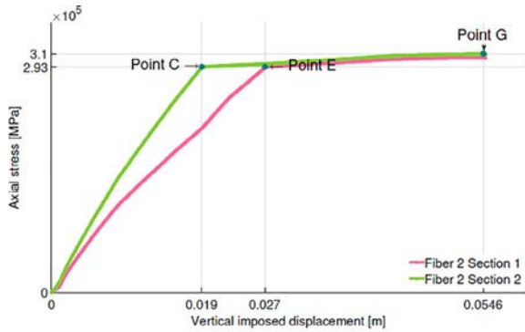
(a) Upper steel of FCQ element 2
