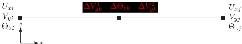
Fig. 1. Timoshenko FCQ beam [23].
