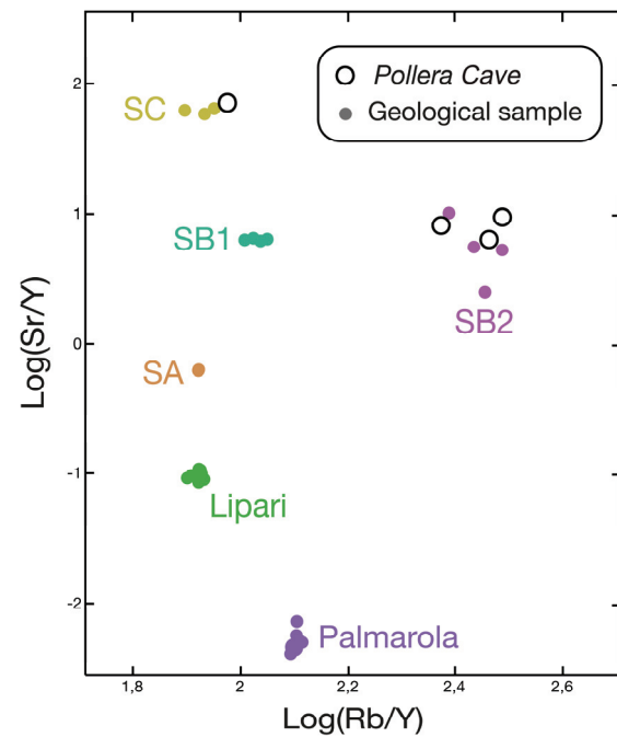
Fig. 5.: Bivariate plot comparing logarithmic ratios determined by EDXRF for the four obsidians samples from Pollera Cave and the different sources of Lipari, Palmarola, and Sardinia.
