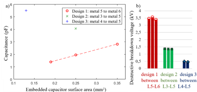
Fig. 10. High voltage embedded capacitor integration measurements for the proposed method (a) capacitance (b) breakdown voltage (L3 to L6 are the metal layer of the technology).
