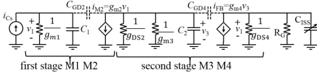
Fig. 8. Small signal analysis of the AGD current mirrors during dv/dt phase.
