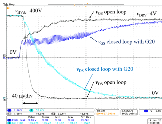
Fig. 6. Experimental results with the CMOS AGD in the 400V DC bus voltage. With the closed-loop, the dv/dt is attenuated from 45V/ns to 6.6V/ns.
