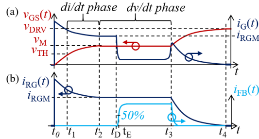
Fig. 2. Qualitative waveforms for gate voltage and currents with the AGD during turn-on (closed-loop). (a) Current and voltage at the power gate and (b) currents being supplied and sunk simultaneously by the AGD.
