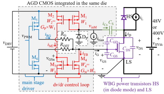
Fig. 1. CMOS AGD topology in a transistor level schematic.
