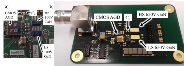
Fig. 4. AGD in a half bridge configuration for test in double pulse for (a) 4-layer board with 48V DC bus voltage with 100V GaN EPC 2001C device. (b) 6-layer board with 400V DC bus voltage with 650V GaN systems GS66508T devices.
