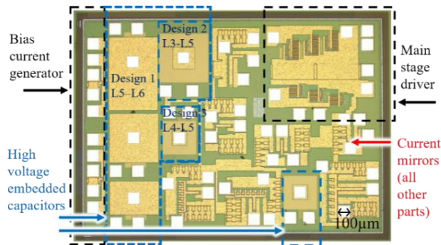
Fig. 3. Optical microscope photograph of the CMOS AGD test chip built in 0.18µm technology.
