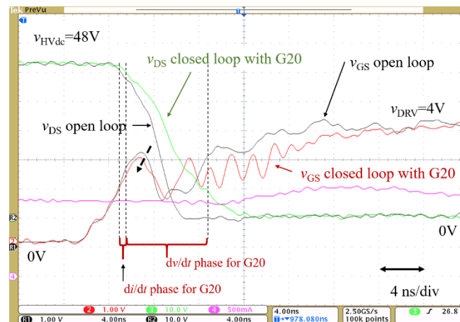
Fig. 5. Experimental results with the CMOS AGD in the 48V DC bus voltage. With the closed-loop, the dv/dt is attenuated from 15V/ns to 6.3V/ns.
