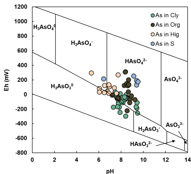
Figure 7: Arsenic Pourbaix diagram showing the As speciation expected for the watertable samples collected in surface water (S) and soil horizons (Hig, Cly or Org) at Centenário farm (see Table 1 for the corresponding total As concentrations). Both, pH and Eh were measured in the field, under N_2 flux.
