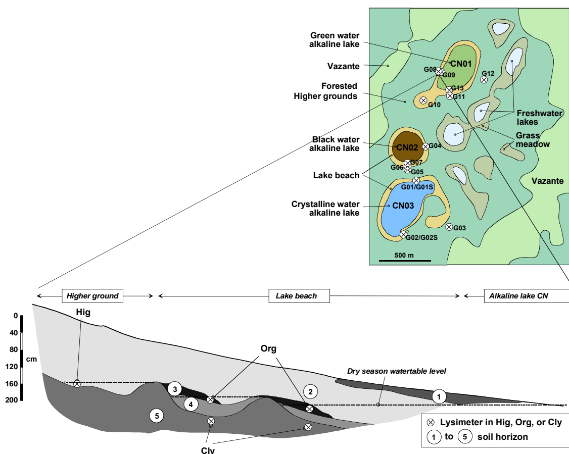
Figure 2: Centenário study site showing a representative landscape, and a standard soil sequence around saline alkaline lakes; see text for soil horizons description. ⊗ denotes the location of the lysimeters in the perched water table.
