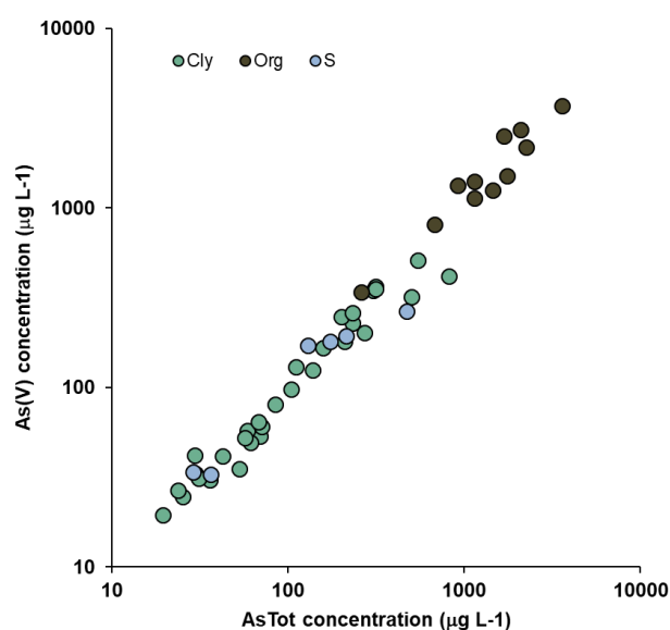
Figure 8: Concentration of As(V) vs Total As in water samples from Centenário farm: S (surface water), Cly (water from clay horizons), Org (water from organic horizons). In water samples from the higher grounds (Hig), As(V) contents were below the limit of quantification.
