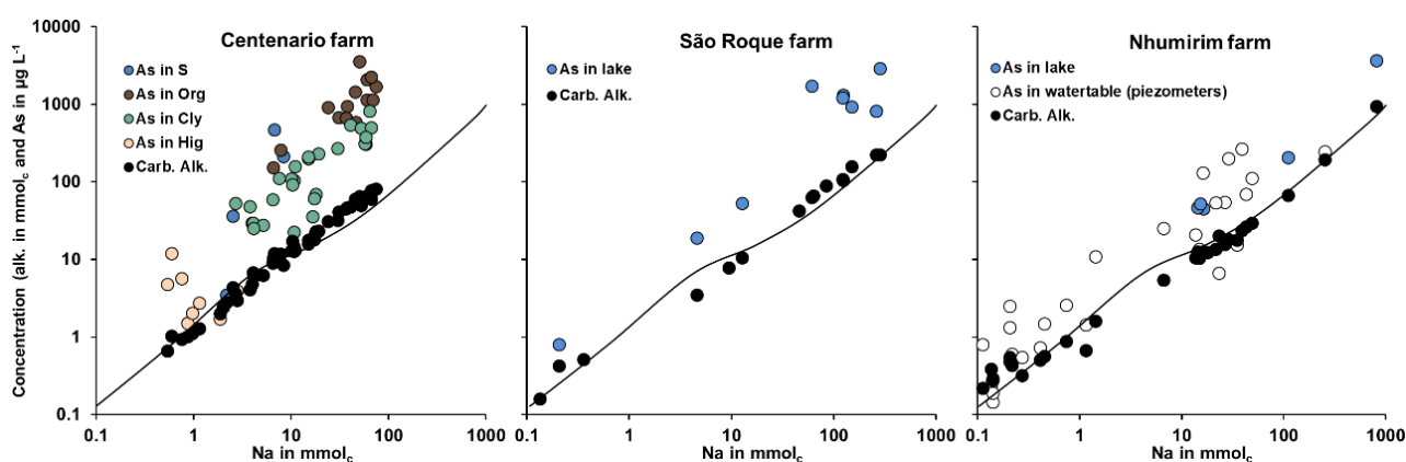
Figure 6: Arsenic and carbonate alkalinity in concentration diagrams based on Na contents (Centenário, São Roque and Nhumirim farms). The solid line denotes the regional Alk-Na relationship established by Furian et al. (2013) from 147 samples of surface water.
