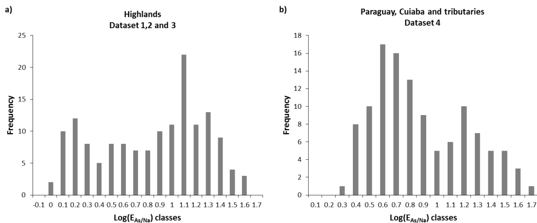
Figure 5: Frequency distribution of \text{log}(E_{As/Na}) a) on the highlands and b) in the floodplain of the UPRB.
