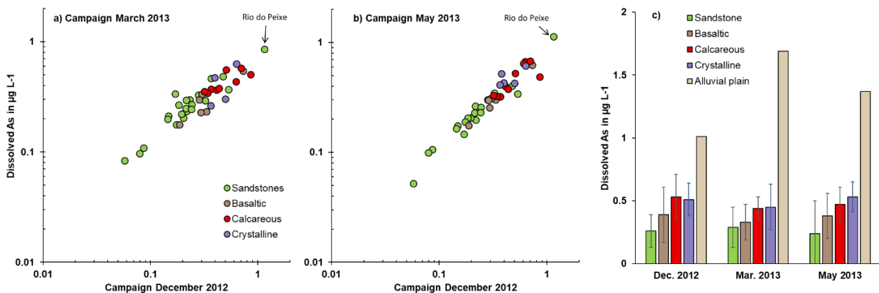
Figure 3: Total dissolved As contents (a and b), mean value and standard deviation (c) in rivers on the highlands and alluvial plain (Nabileque River) during 3 campaigns in 2012-2013.
