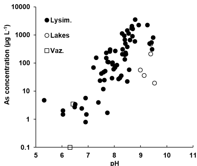
Figure 9. Dissolved As concentration vs pH in lysimeters, lakes and vazante at Centenário farm.
