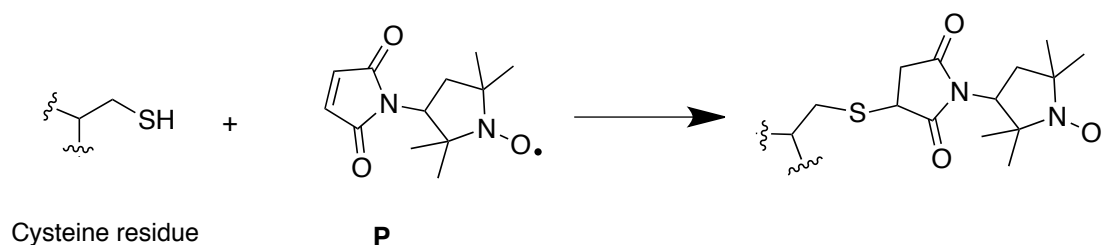
Scheme 2. Cysteine-labeling reaction with proxyl ( P )
