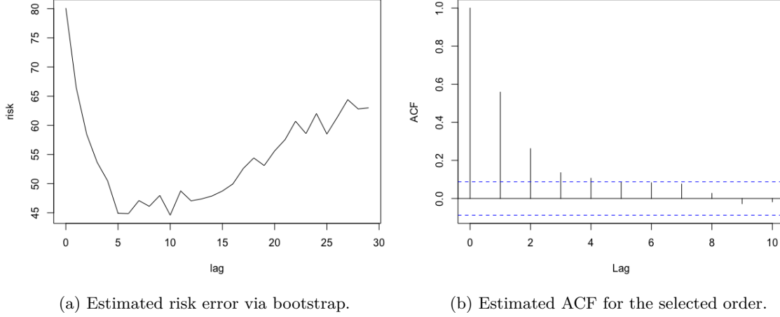
Figure 3: Plots output by slm for the kernel method with bootstrap selection of the order.
