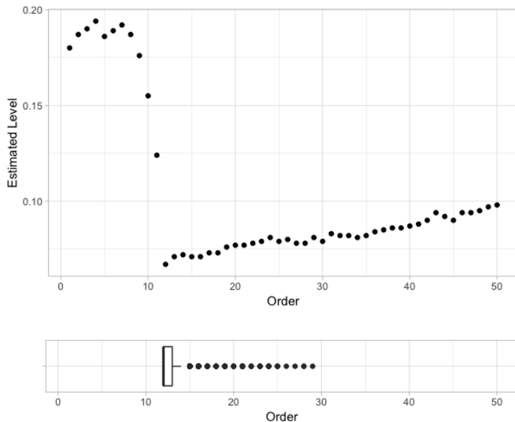
Figure 5: Estimated level of the test according to the order of the fitted AR process on the residuals (top) and boxplot of the order selected by AIC, over 1000 simulations. The data has been simulated according to Model (5) with \beta_1 = 3 and \beta_2 = \beta_3 = 0 , with n = 1000 .
