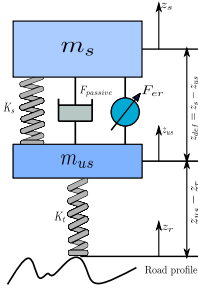
Fig. 1. 1/4 car model with semi-active suspension
