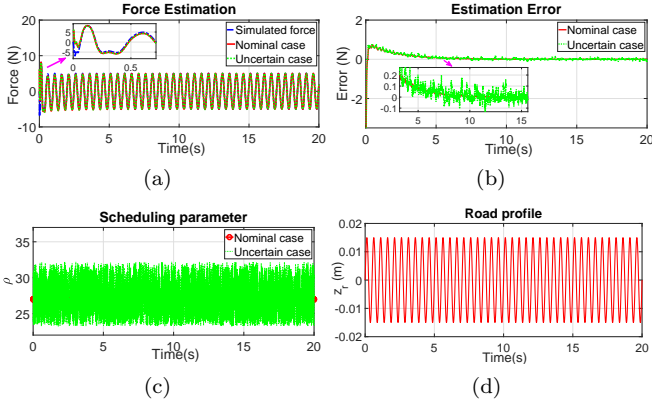
Fig. 3. Simulation scenario 1: (a) Damping force estimation, (b) Estimation error, (c) Scheduling parameter, d) road profile
