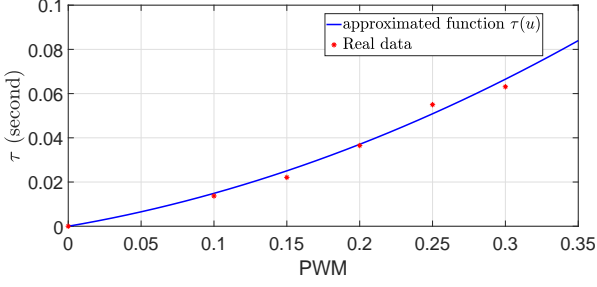
Fig. 2. The relation between \tau and u
