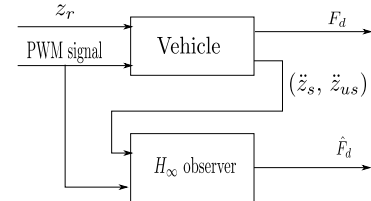
Fig. 6. Block diagram for implementation of the \mathcal{H}_\infty damper force observer
