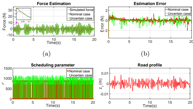
Fig. 4. Simulation scenario 2: (a) Damping force estimation, (b) Estimation error, (c) Scheduling parameter, d) road profile
