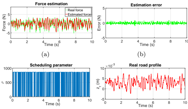
Fig. 8. Experiment 2: (a) Damping force estimation, (b) Estimation error, (c) Scheduling parameter, d) road profile
