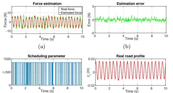
Fig. 7. Experiment 1: (a) Damping force estimation, (b) Estimation error, (c) Scheduling parameter, d) road profile
