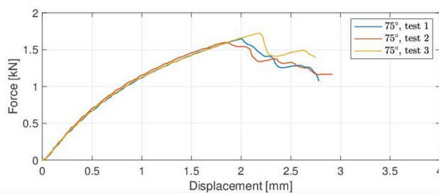
Fig. 47: Series of force-displacement curves for 25 mm specimens and 75° fiber orientation.
