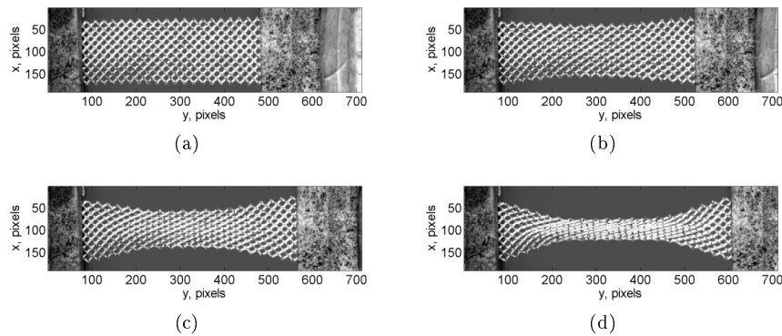
28 Fig. 65: Gray level images of the pantograph in the reference configuration (a), 29 17th (b), 34th (c) and 51st (d) loading steps 30
