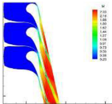
Fig. 1. Mach number distribution for a viscous deterministic calculation at nominal operating conditions
