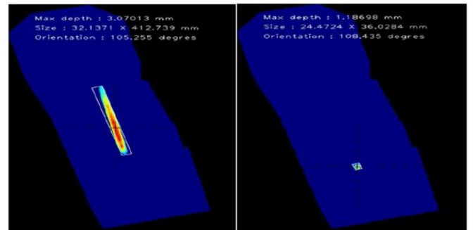
Fig. 18. The algorithm provides shape, size and depth of surface imperfections with visual color representation to help the human operator.
