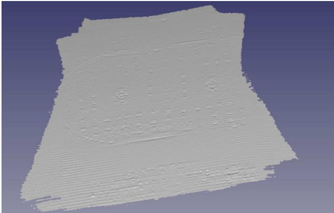
Fig. 16. Tridimensional scan of the static port area, the texture is visible.
