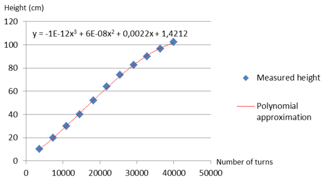
Fig. 12. Curve representing the elevator height in function of the number of motor turns.
