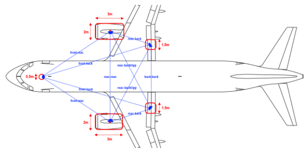
Fig. 8. Items used in the 2D pose estimation process.
