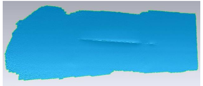
Fig. 17. Tridimensional scan of the aircraft, a crack and a bump are visible.
