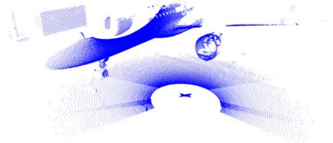
Fig. 6. Robot is located in front left of the aircraft in an outside environment. 3D data is acquired with a laser range finder moved thanks to a PTU.
