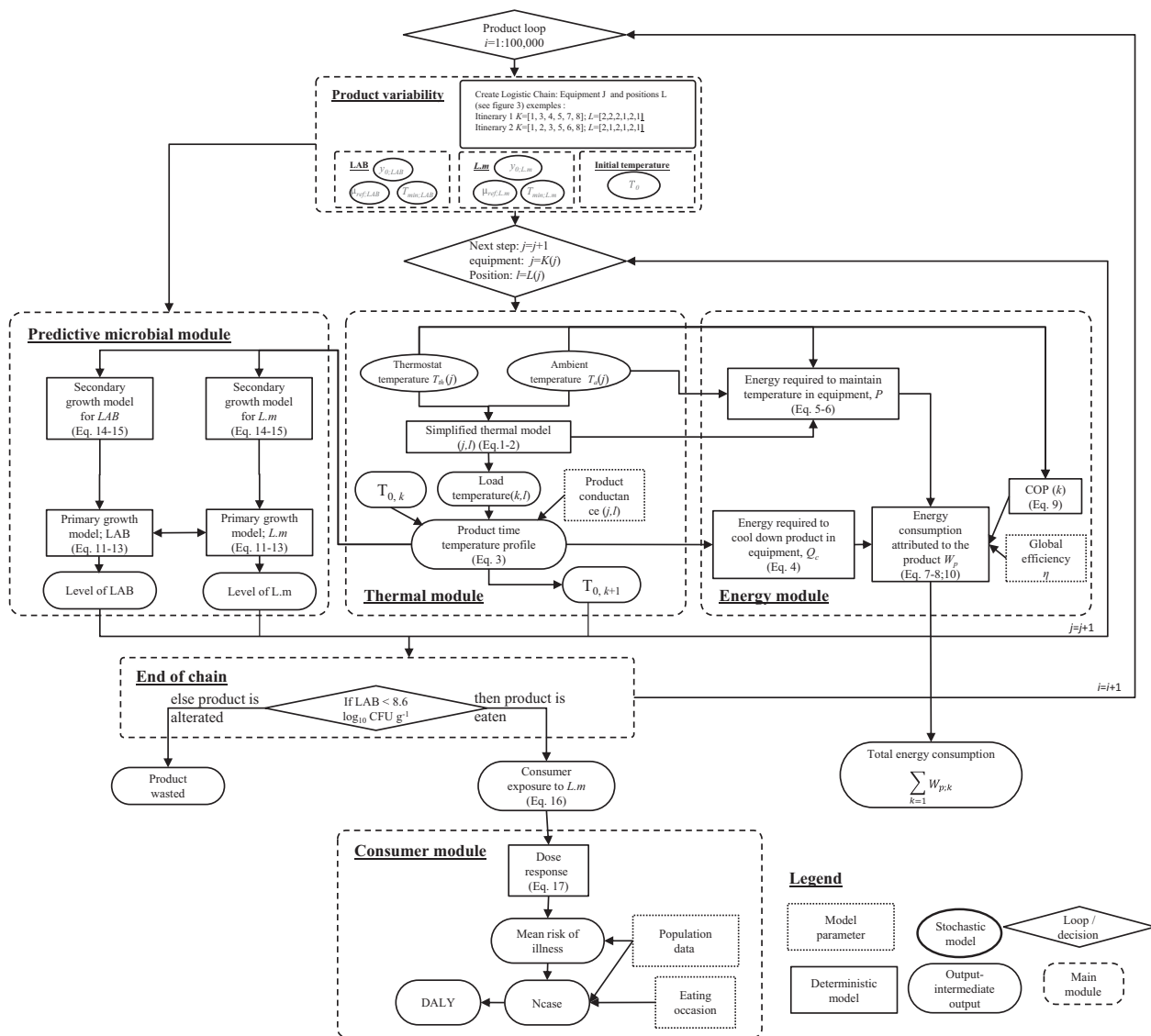
Fig. 1. Model overview.
