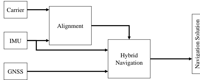
Fig. 2. Navigation architecture
