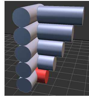
Figure 20: Side view of two printed walls at a junction. Note the progressive, downward erosion of the right part. At a junction between walls we take special care to avoid over-extrusion. Child walls do not reach the parent wall but stop before, taking into account extrusion width. Only the first layer (in red) starts from the actual branching point to allow some overlap and ensure adherence.
