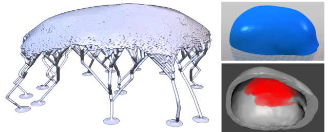
Figure 8: Pillar structure supporting an hollowed skull top model (top right). The red areas along the cavity roof (bottom right) cannot print without support. The pillars are generated by Autodesk Meshmixer (Schmidt and Umetani [SU14]). We set support density to match our support requirements as defined in Section 3.2. Note how pillars fuse below the overhanging surface producing a compact, slow-to-print geometry. Note that the pillars are also quite unstable and subject to torque (see Figure 2 of [DHL14] for details). Model: www.thingiverse.com/thing:4378 by ssd .
