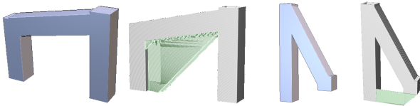
Figure 25: Left: Low angle, flat overhang areas mislead our wall direction heuristics, generating suboptimal supports. Right: Overhang area located far away from the rest of the model and close to the bed. Our method connects the support for that overhang to the post on the left, using up a lot of material. A pillar would use much less material here.
