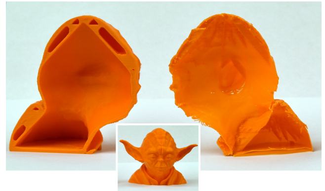
Figure 23: Printing the Yoda model. Left : Hollowed by support-free hollowing [WLW* 18]. Right : Printed with our method and cut open with a blade (hence the raw outline). Center : Result before cut-out. We did not add external supports which explains small defects around the ears.
