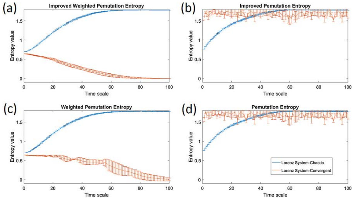
Fig. 4. Results of the four entropy algorithms ( d=3 and l=1 ) on the chaotic and convergent signals generated by the Lorenz System (a) mvIWPE; (b) mvIMPE; (c) mvMWPE; (d) mvMPE.
