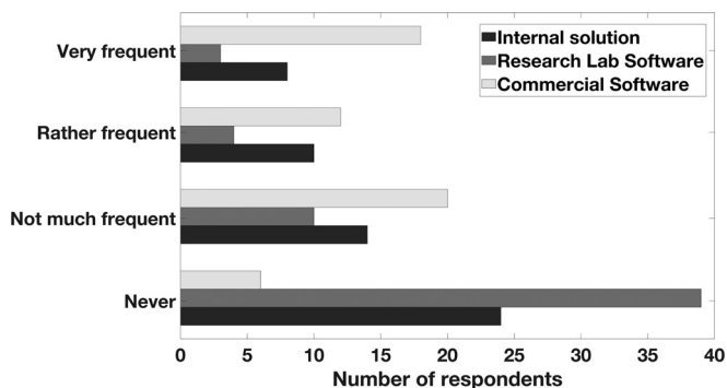
FIG. 3. Method of creation of acoustical models used by respondents to the questionnaire (Light Grey: commercial software, Dark Grey: research laboratory software; Black: internally developed algorithms).
