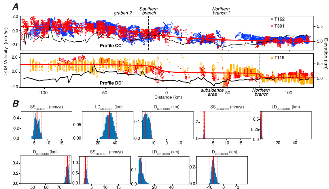
Figure 8. Inversion model and results for the two profiles CC' and DD' across the Jinsha suture defined in Figure 3. (a) Line-of-sight (LOS) velocities (cyan, blue, red, and orange points) along the four swath profiles with average model obtained in red and topography in black. (b) Posterior marginal PDF (blue histograms) with average posterior models (red vertical lines) and boundaries corresponding to the uniform prior distributions.
