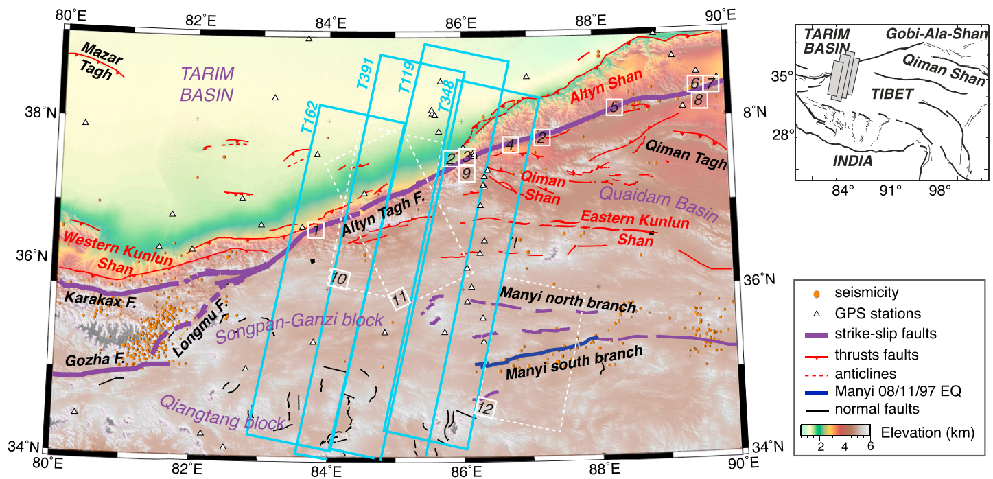
Figure 1. Seismotectonic setting of the Altyn Tagh Fault system superimposed on Digital Elevation Model of the Shuttle Radar Topography Mission (Farr & Kobrick, 2000). Fault traces are modified from Van Der Woerd et al. (2002) and Replumaz and Tapponnier (2003). Orange dots show the seismicity from 1992 to 2014 from USGS. Black triangles are GPS stations from the Observation Network of China (Wang et al., 2017) and from the GPS transect of He et al. (2013). Surface traces of four overlapping Envisat descending tracks 162, 391, 119, and 348 used in this study are in cyan. Previous interseismic slip rate investigations include Quaternary time scale measurements from offset risers and glacial features from (1) Peltzer et al. (1989) (~20–30 mm/yr), (2) Mériaux et al. (2004) ( 27 \pm 7 mm/yr), (3) Cowgill (2007) ( 9.4 \pm 2.3 ), (4) Gold et al. (2009) (~7–17 mm/yr), (5) Cowgill et al. (2009) ( 11.5 \pm 2.5 mm/yr), and (6) Mériaux et al. (2012) ( 14 \pm 1 mm/yr); paleoseismic measurements from (7) Washburn et al. (2001) (~10–20 mm/yr); GPS transects measurements from (8) Wallace et al. (2004) ( 9 \pm 4 mm/yr) and (9) He et al. (2013) ( 9 \pm 4 mm/yr); and interferometric synthetic aperture radar studies across the Altyn Tagh Fault from (10) Elliott et al. (2008) ( 11 \pm 10 mm/yr) and from (11) Zhu et al. (2016) ( 8 \pm 0.7 mm/yr), as well as across the MF, which broke during the 1997 M 7.6 earthquake (blue line), from (12) Bell et al. (2011) ( 3 \pm 2 mm/yr).
