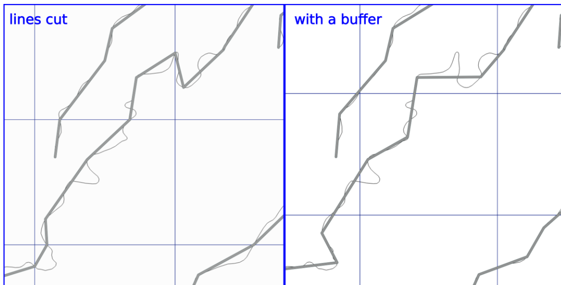
Figure 8. Differences in the cartographic output for Visvalingam-Whyatt simplification of rivers when using a buffer for context, or when cutting lines.
